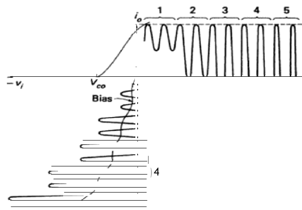
FIGURE 7 Amplitude limiter transfer characteristic.
