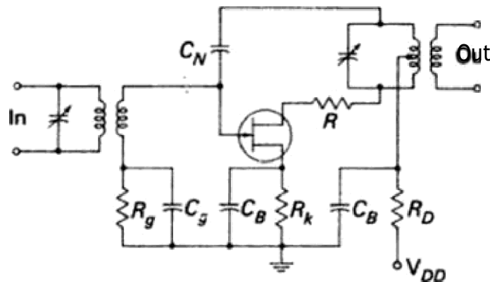
FIGURE 6 Amplitude limiter.
