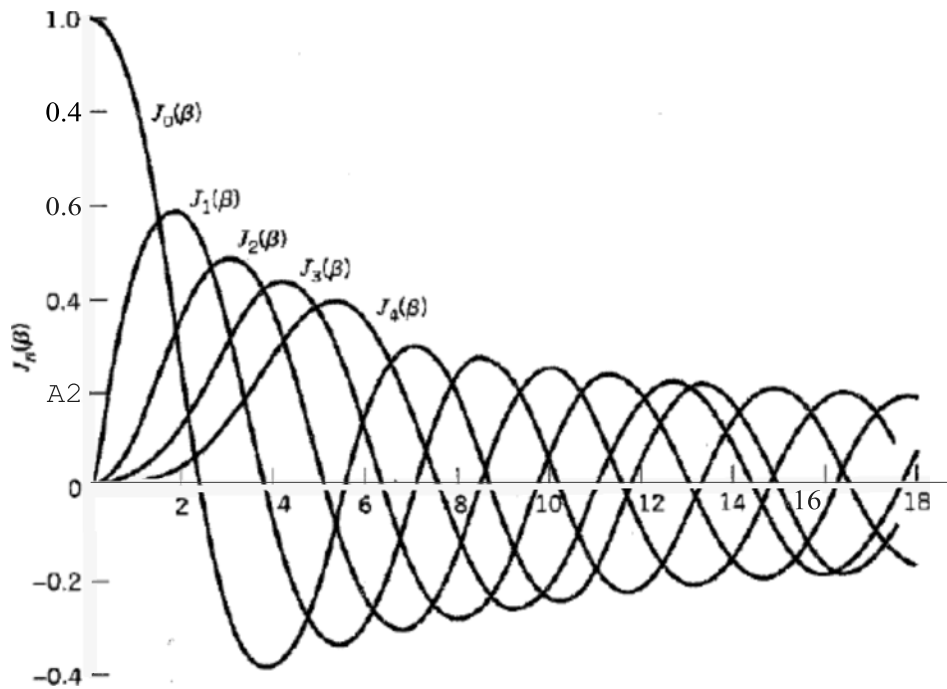
Figure 5.3 Plot of Bessel function as a function of modulation index.
