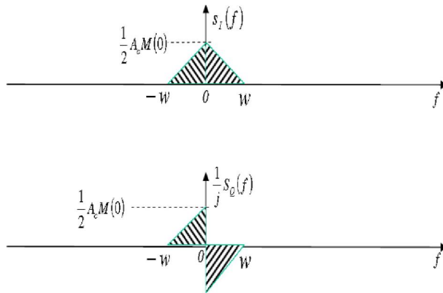
Figure 14 : Spectrum of quadrature component of SSBSC-USB
