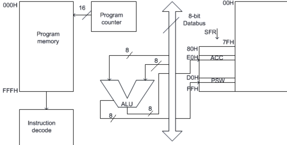
Fig 4.4 : Basic 8051 Architecture
