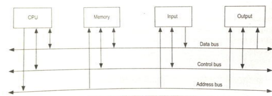
Fig.1 Microprocessor-based system
