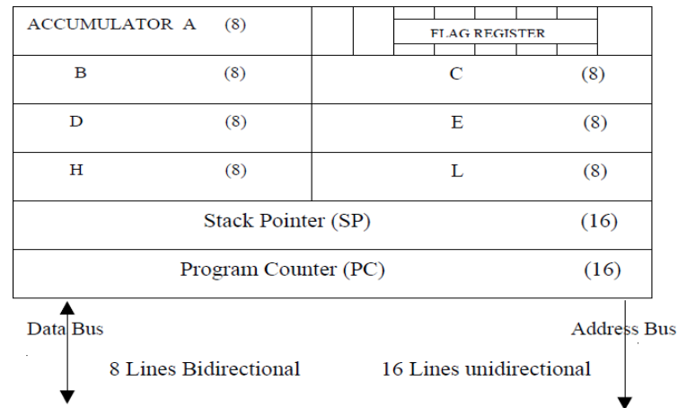
Fig. 3 Register organisation
